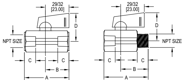
Female X female connection SMV2-WFX
